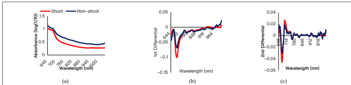
Figure-5. The light absorbance of the shoot and non-shoot buds for the ‘Miyabi Fuji’ seven days before bud burst. The 1 st Differential and 2 nd Differential on the visible/near-infrared spectrometer; (a) Absorbance (log(1/R)); (b) 1 st Differential and (c) 2 nd Differential.
