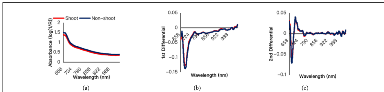
Figure-6. The light absorbance of the shoot and non-shoot buds for the ‘Orin’ seven days before bud burst. The 1 st Differential and 2 nd Differential on the visible/near-infrared spectrometer; (a) Absorbance (log(1/R)); (b) 1st Differential and (c) 2nd Differential.
